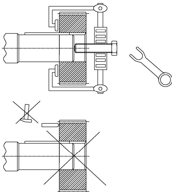
DISMOUNTING
