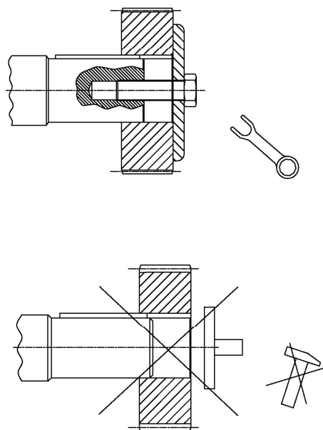
MOUNTING
